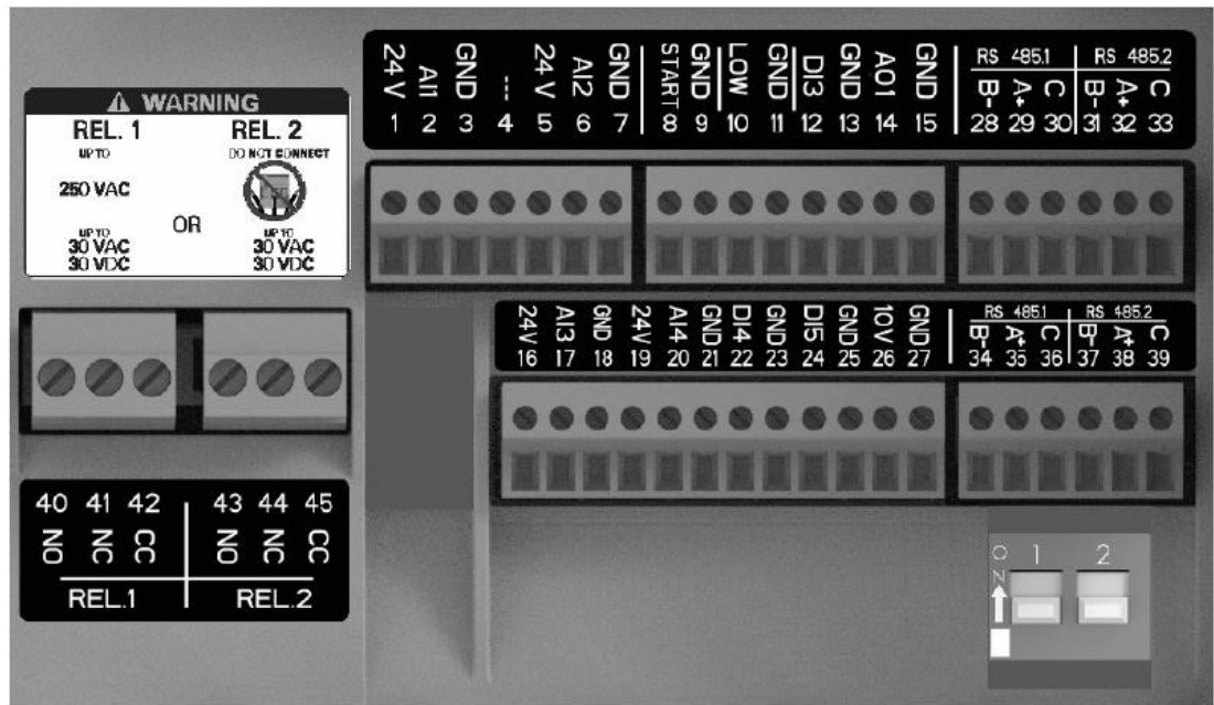
Figure 8: Raccords auxiliaires
