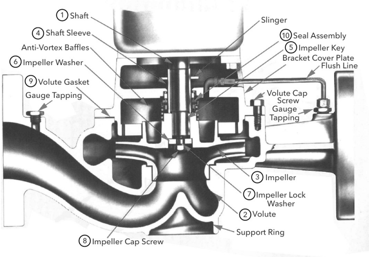
Standard Mechanical Seal
