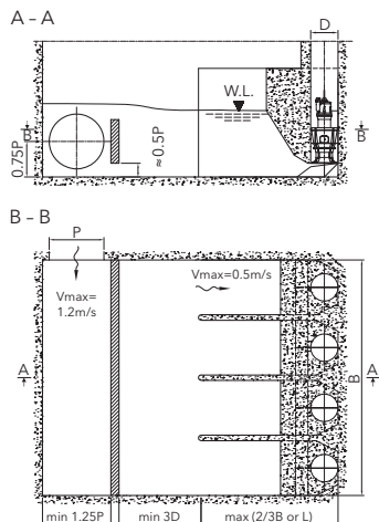
Stations with low level side inlet (max 4 pumps)
