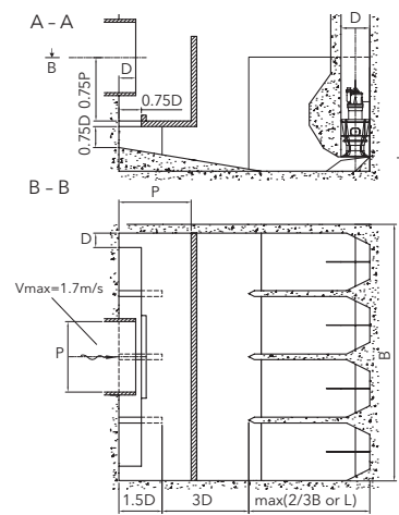
Stations with high level front inlet (max 4 pumps)
