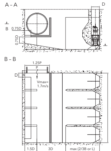
Stations with high level side inlet (max 4 pumps)
