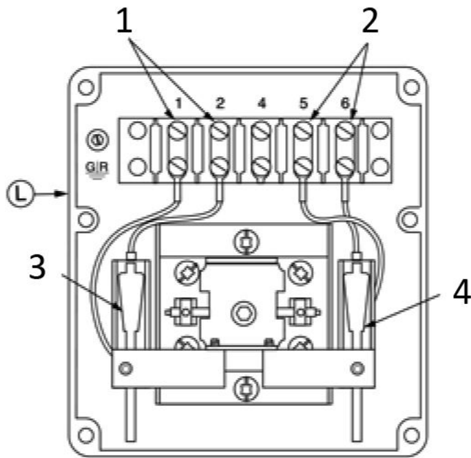
Figure 15: Automatic reset model 159S
