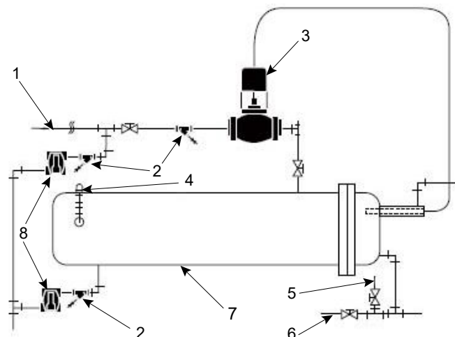
Figure 1: Hot water converter
