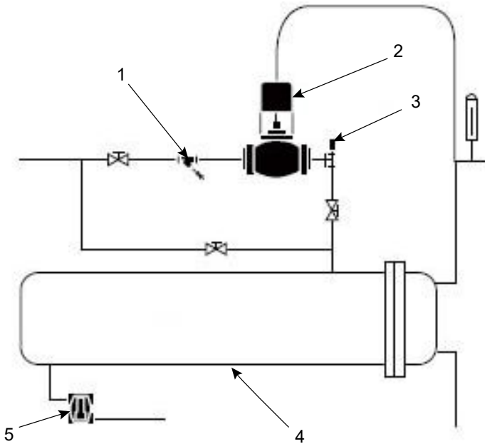
Figure 3: Tankless water heater
