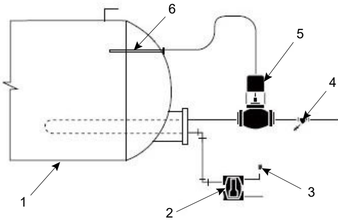
Figure 2: Storage tank water heater
