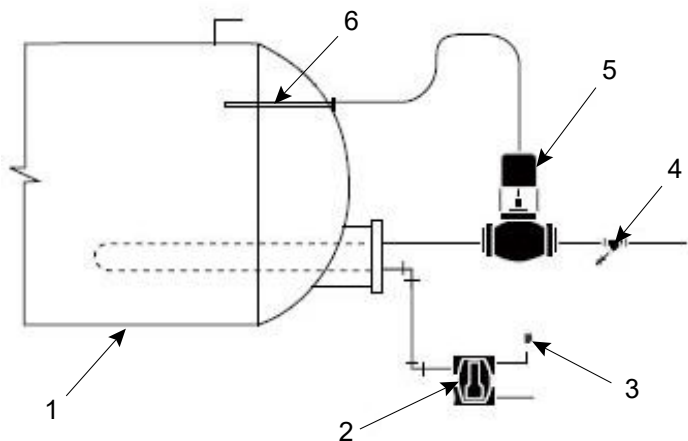
Figure 2: Chauffe-eau à accumulation
