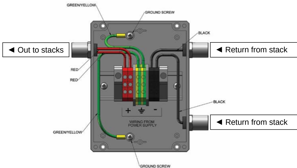
Figure 3-5: Inside the VNX Junction Box (2-stack module) Max, Mini, Ultra have one set of red/black/green wires
