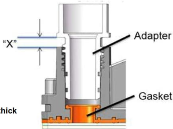
Figure 3-4: Proper Tightening of VNX Piping Adapter
